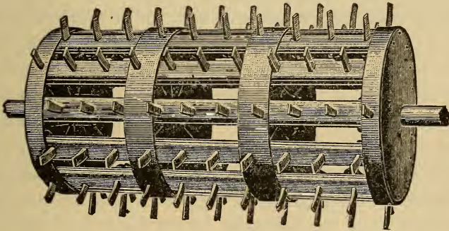
FIG. 68.—REEVES STANDARD CYLINDER.
